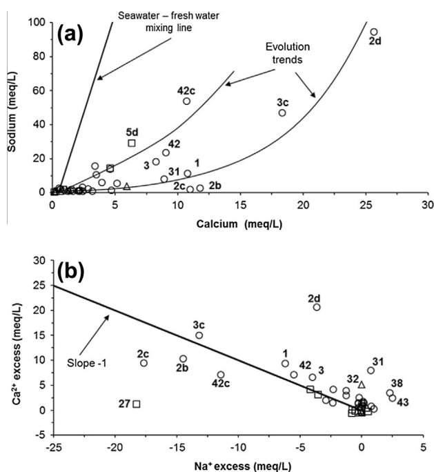
Fig. 10. Results from Lower Tagus–Lower Sado basin: (a) sodium vs. calcium; (b) calcium excess vs. Na excess in Sado–Tagus groundwaters. The replacement of \text{Na}^+ by \text{Ca}^{2+} through ion exchange is triggered by seawater (symbols as in Fig. 7).
