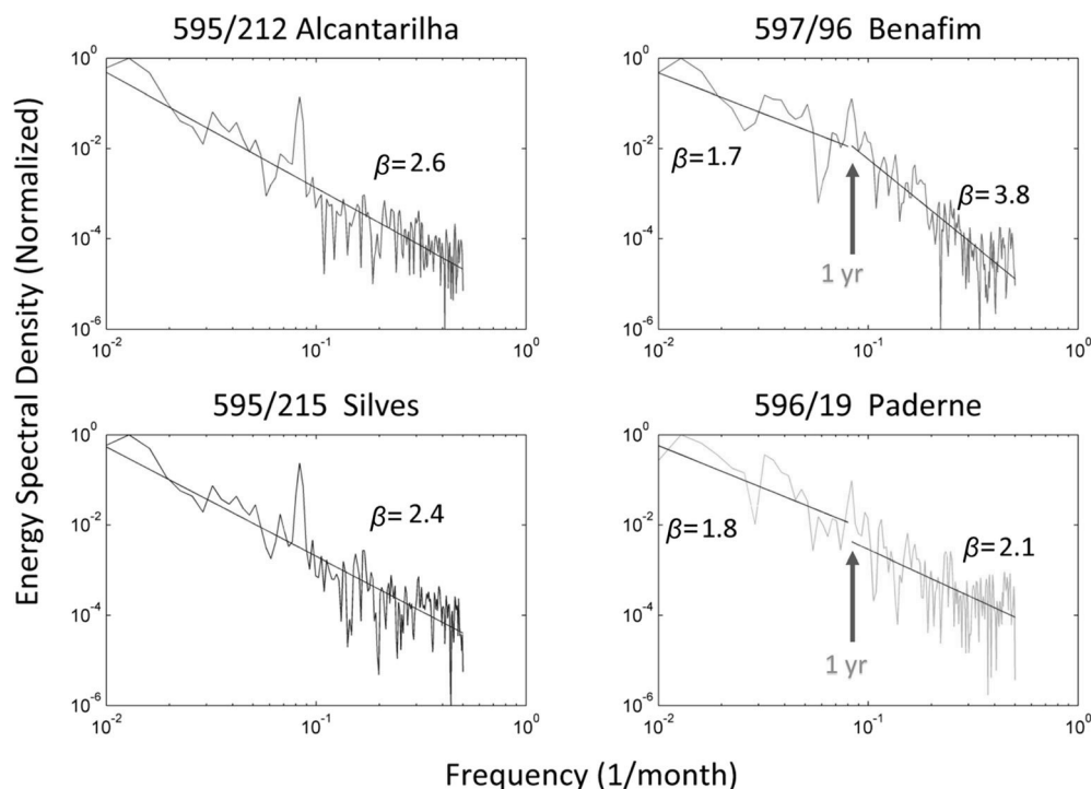
Fig. 6 Energy (power) spectra of the four groundwater level records in a log-log plot. The slopes of the lines, computed from linear regression, correspond to estimates of the empirical \beta exponents defining scaling regimes
