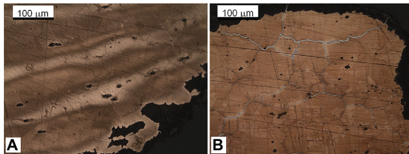
Fig. 9. OM images of VNSP146D (As = 2.04%) revealing the elongation of the segregation bands (A) and VNSP180E revealing the As-rich \gamma phase following the grain boundaries (B), (all BF illumination, etched).
