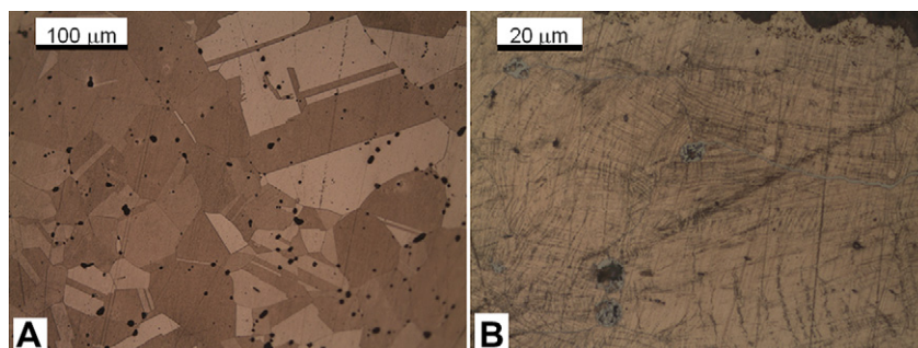
Fig. 5. OM images of VNSP133C (As < 0.10%) revealing annealing twins (A) and VNSP0251 (As = 3.37%) revealing slip bands (B), (all BF illumination, etched).
