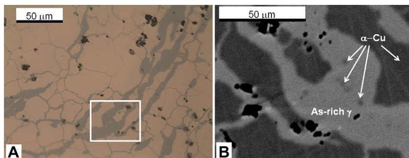
Fig. 10. A: OM image of VN2P148D ( As = 9.13\% ) (BF illumination); B: SEM-BSE image with the region marked on the OM image showing the EDS identification of: As-rich \gamma phase, \alpha -Cu phase and \alpha -Cu islands.
