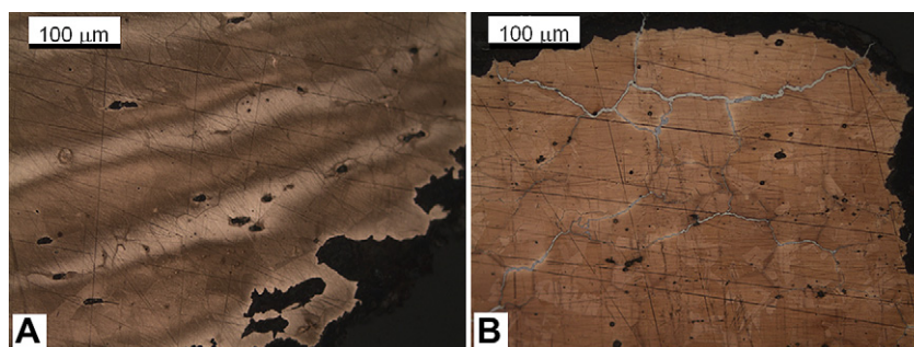
Fig. 9. OM images of VN2P146D ( As = 2.04\% ) revealing the elongation of the segregation bands (A) and VN2P180E revealing the As-rich \gamma phase following the grain boundaries (B), (all BF illumination, etched).
