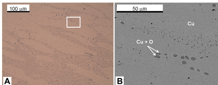
Fig. 8. A: OM image of VN2P268D ( As < 0.10\% ) (BF illumination); B: SEM-BSE image with the region marked on the OM image showing the EDS identification of the \alpha -Cu phase and Cu_2O inclusions (Cu + O).
