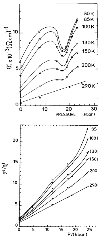
Figure 13. Pressure dependence of the conductivity of TTF–TCNQ showing the drop of metallic conductivity in the commensurability domain. The transverse conduction (bottom) remains unaffected by commensurability. (Reprinted with permission from ref 25. Copyright 1982 Taylor and Francis ( http://www.tandf.co.uk/journals )).
