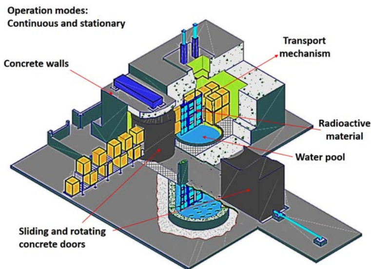
FIG. 6.1. A typical panoramic, wet storage gamma irradiation facility (courtesy of MDS Nordion, Canada).
