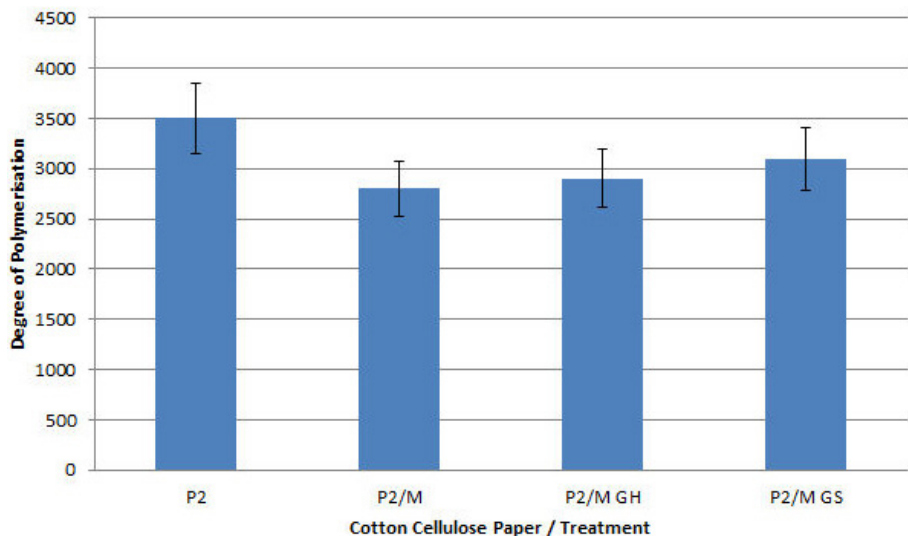
FIG. 12.4. The degree of polymerization of the cotton cellulose paper before mould and irradiation (P2), after infection by mould and dry cleaning (P2/M), and after infection by mould and irradiation using maximum 10 kGy and subsequent surface cleaning and flattening (P2/M GH and P2/M GS).
