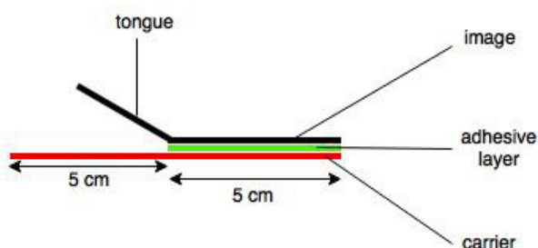
FIG. 7.8. Set-up for testing the delamination of film materials. The tensile test equipment was put on the tongue (artificially created on the sample of the photographic materials) and on the carrier, which was a paper based layer.
