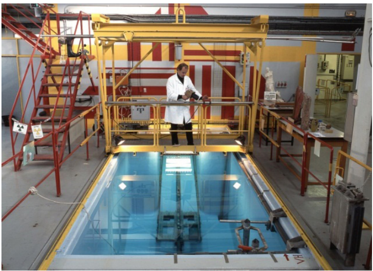
FIG. 26.1. The ARC-Nucléart irradiation facility.
