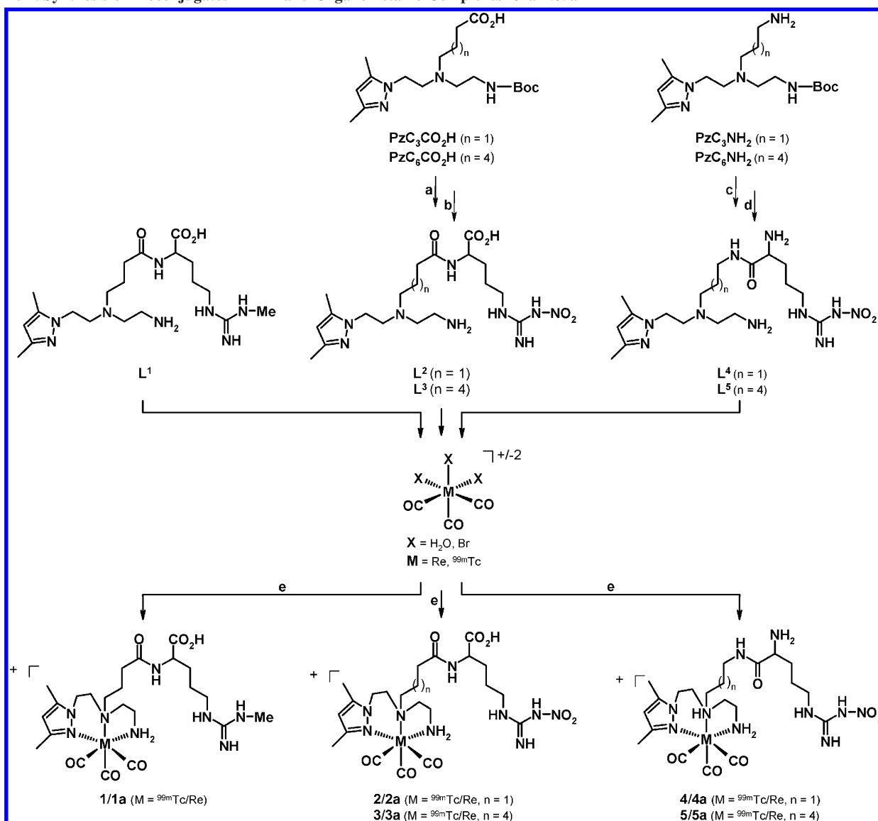
Scheme 1. Synthesis of Bioconjugates L^2 – L^5 and Organometallic Complexes 1/1a – 5/5a a
