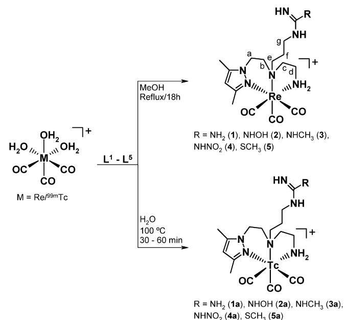
Scheme 2. Synthesis of the M(I)-tricarbonyl complexes 1/1a – 5/5a . Identification system for NMR assignments is displayed.
