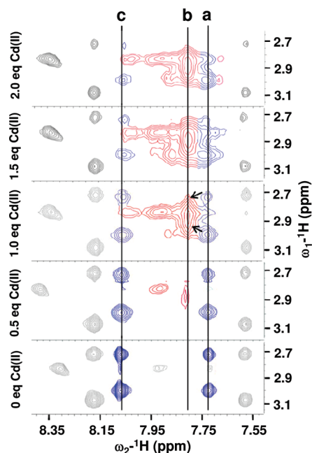
Figure 7. Sections of ^1\text{H} - ^1\text{H} NOESY spectra of 3.25 mM ( GRANDL12AL16CL26AL30C ) 3 as a function of added equivalents of Cd(II) at pH 6.0. Peak at 7.91 ppm corresponds to \text{H}^{\text{N}} of E21 and other peaks displayed in gray correspond to interresidue NOEs ( \text{H}^{\text{N}}_i - \text{H}^{\beta}_{i+i} ) (see text for full description). Colored peaks correspond to intraresidue NOEs of the amide protons ( \text{H}^{\text{N}} , vertical axis) and the \beta -methylene protons ( \text{H}^{\beta} , horizontal axis) of Cys: (a) \text{H}^{\text{N}}_{16} - \text{H}^{\beta}_{16} for GRANDL12AL16CL26AL30C ; (b) \text{H}^{\text{N}}_{16} - \text{H}^{\beta}_{16} for [\text{Cd}(\text{II})(\text{H}_2\text{O})]^{16}[\text{apo}]^{30} ( GRANDL12AL16CL26AL30C ) 2- ; and (c) \text{H}^{\text{N}}_{30} - \text{H}^{\beta}_{30} for GRANDL12AL16CL26AL30C .
