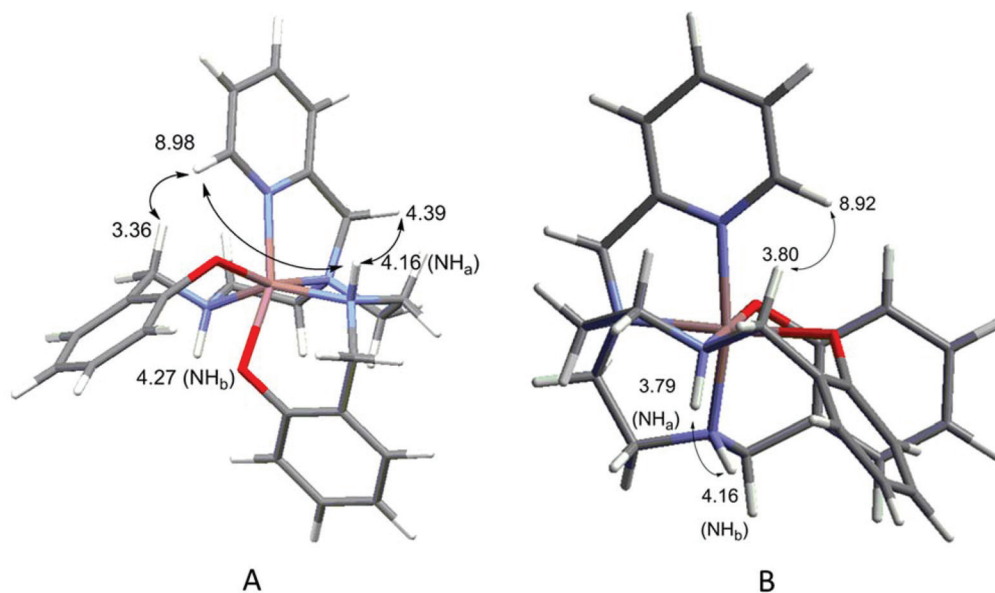
Fig. 5 Relevant NOE enhancements used to confirm the mer - \text{N}_3\text{dien} coordination in isomer A and the fac - \text{N}_3\text{dien} coordination in isomer B of [\text{GaL}^{\text{py},\text{NH}}]^+ in \text{CD}_3\text{CN} .
