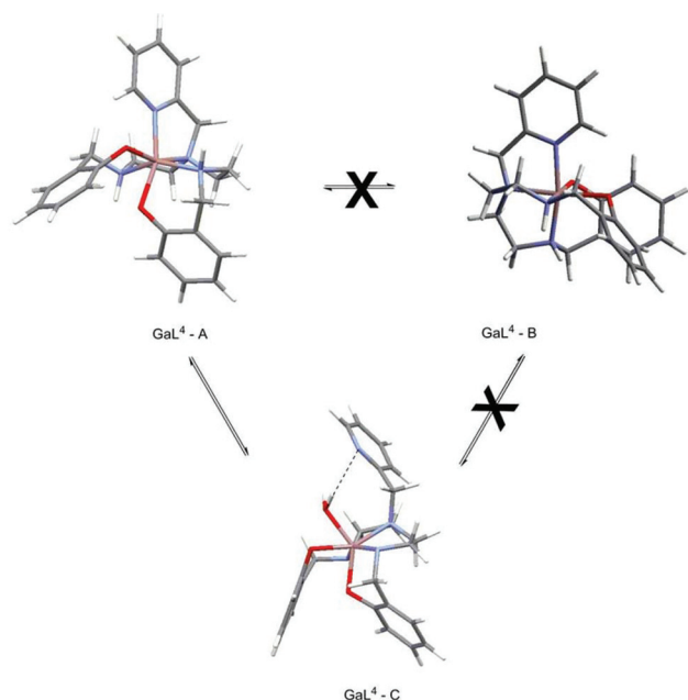
Scheme 3 [\text{GaL}^{\text{py},\text{NH}}]^+ species present in acetonitrile solution.
