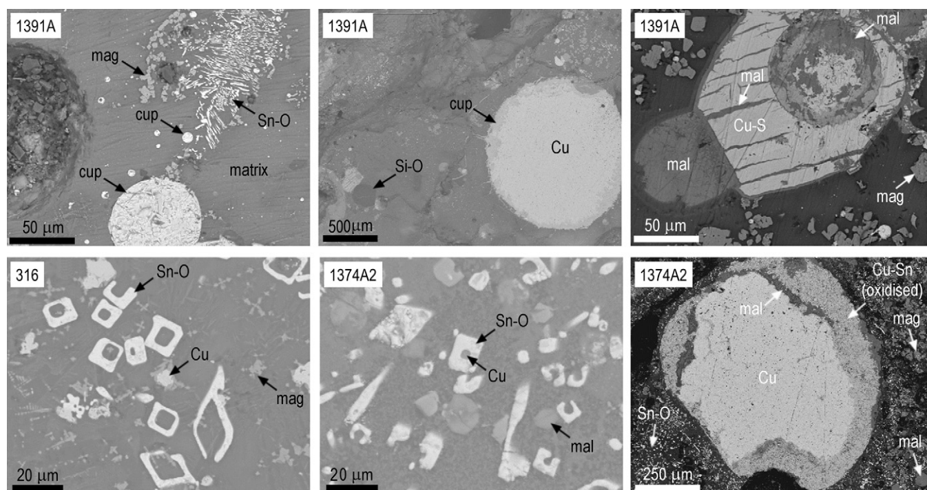
Fig. 6. SEM-BSE images of the slag in crucibles 1391A, 316 and 1374A2.
