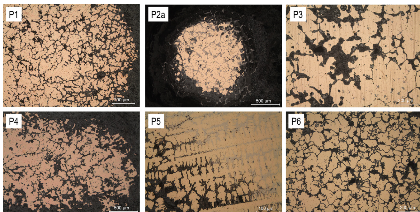
Fig. 8. OM-BF images of metallic prills recovered from the metallurgical workshop at EA5.
