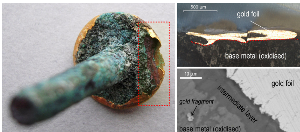
Fig. 10. Image of gilded nail 1495b showing the gold foil over a totally corroded bronze head (OM-BF and SEM-BSE images of contact area between foil and bronze substrate).
