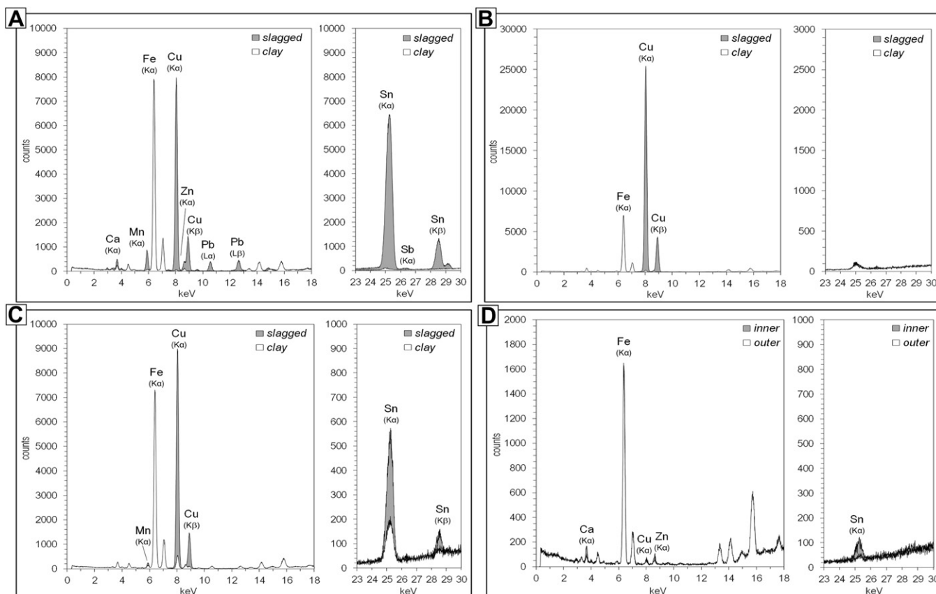
Fig. 4. EDXRF spectra of slagged/inner versus clay/outer surface of the socketed crucible 1374A (A), triangular lip crucible 1374 (B), tuyere 1374 (C) and mould 1432B2 (D).
