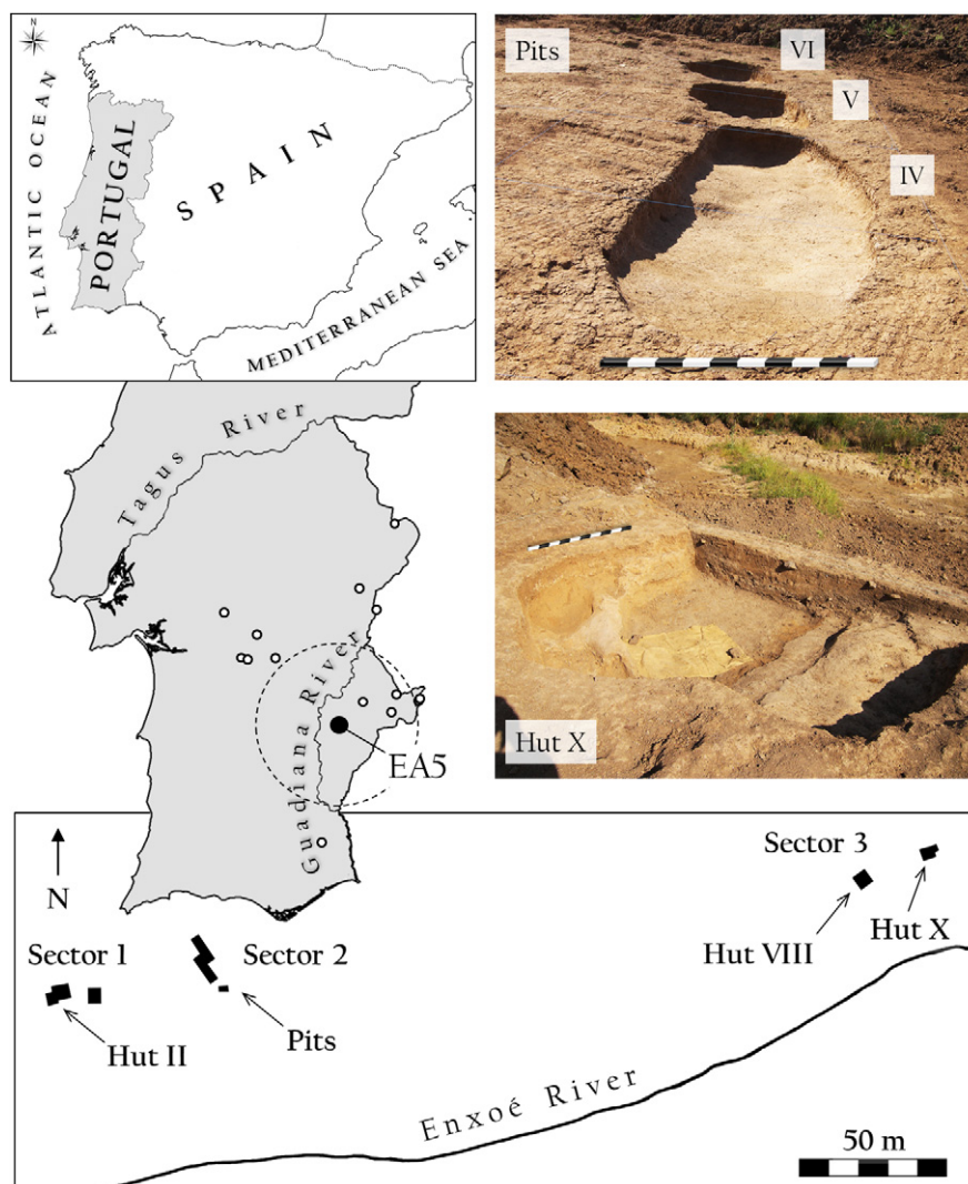
Fig. 1. Location of Entre Águas 5 (EA5) in Southern Portugal (circle equals 100 km), prehistoric copper mines given by Müller et al. (2007), photos of negative structures (pits and hut X; scale equals 1 m) and settlement plan with excavated sectors, huts and pits.
