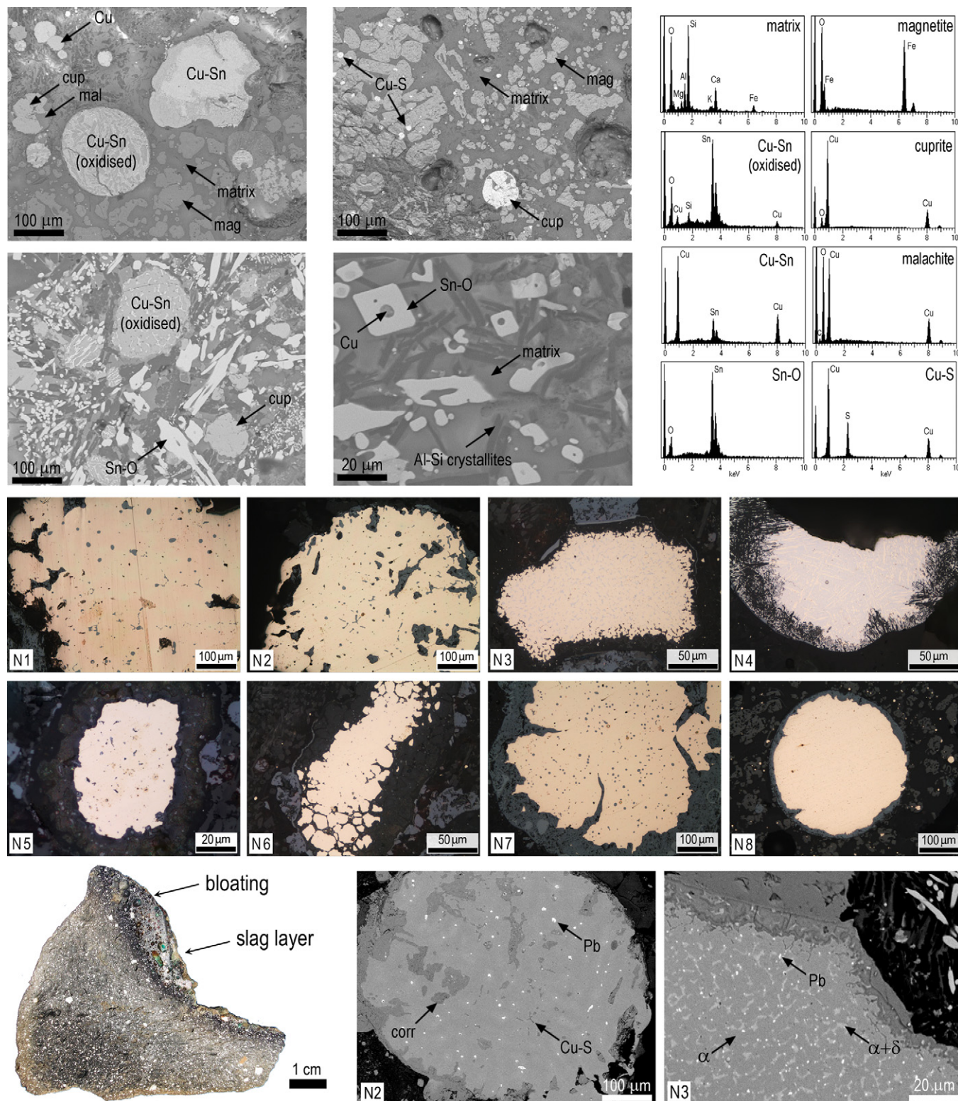
Fig. 5. SEM-BSE and OM-BF images of slag and metallic nodules in crucible 1374A (cross-section evidencing the slag layer and bloating of crucible ceramics).
