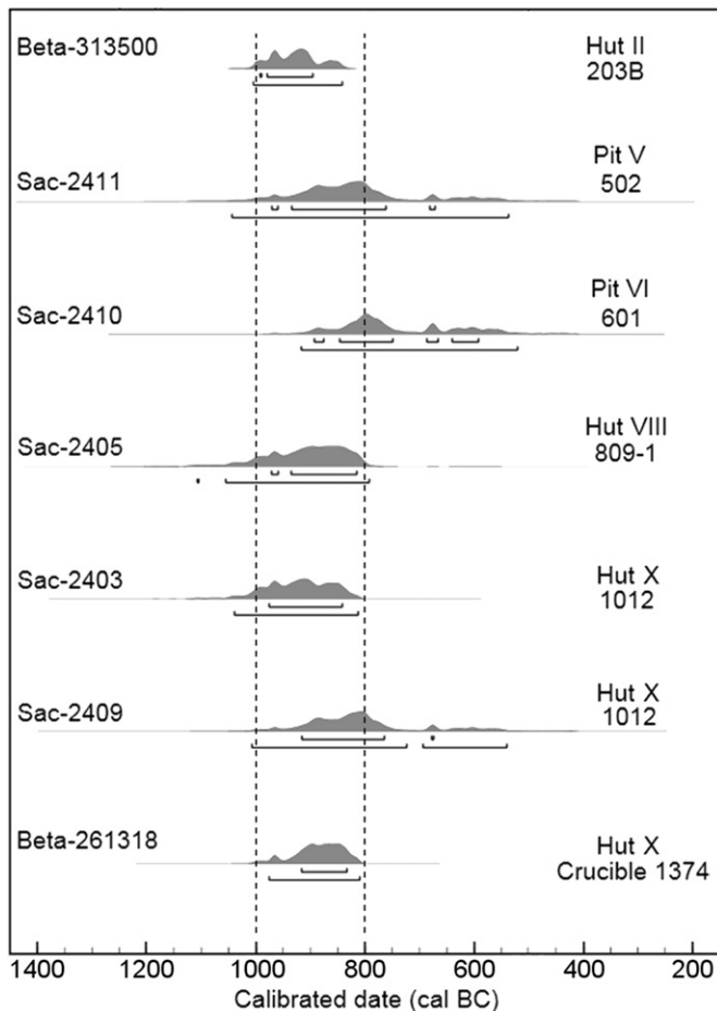
Fig. 2. Radiocarbon calibrated dataset generated by OxCal program (dashed lines are suggested limits for the metallurgical workshop at EA5).
