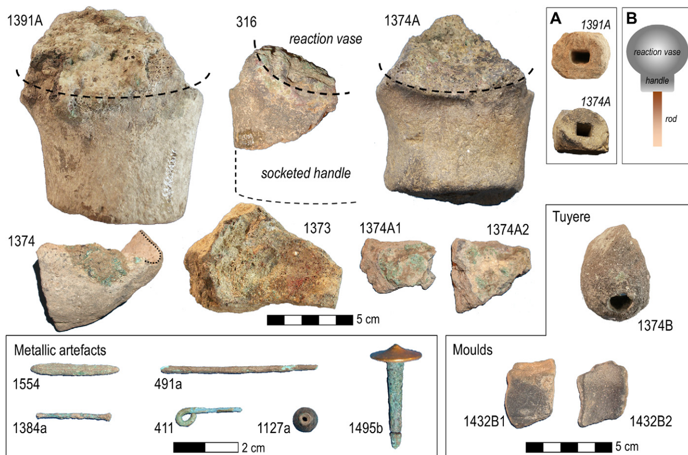
Fig. 3. Production remains and metallic artefacts recovered from the LBA settlement of EA5 (A: sockets from crucibles 1391A and 1374A; B: diagram of socketed crucible with rod).
