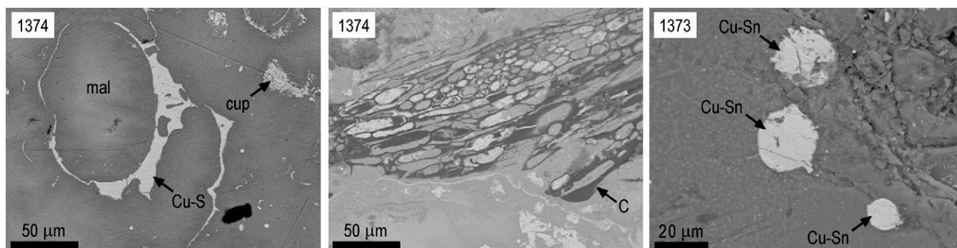
Fig. 7. SEM-BSE images of the slag in crucibles 1374 and 1373.
