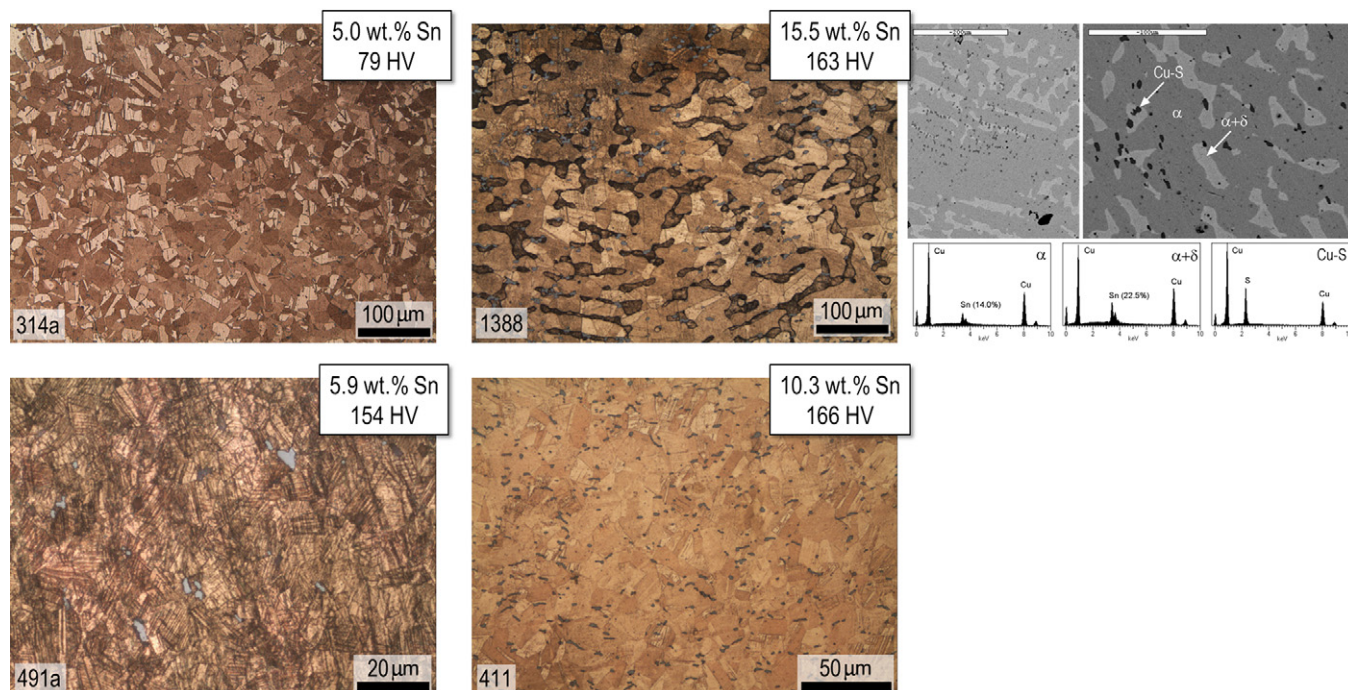
Fig. 9. OM-BF and SEM-BSE images of bronze artefacts recovered from the LBA settlement of EA5.
