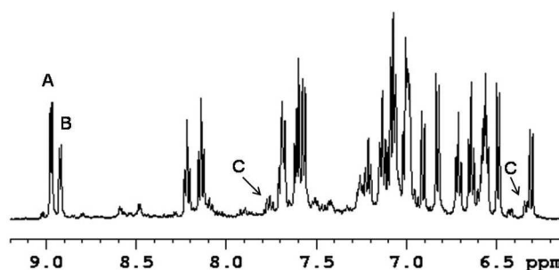
Fig. 4 Aromatic region of the ^1\text{H} spectrum of [\text{GaL}^{\text{py},\text{NH}}]^+ in \text{CD}_3\text{CN} showing the presence of two major isomers A and B in a 1:0.6 ratio. Some of the peaks of the minor species C are also identified.
