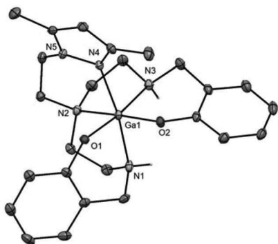
Fig. 1 ORTEP drawing at the 40% probability level for the [\text{GaL}^{\text{pz}^*,\text{NH}}]^+ cation in [\text{GaL}^{\text{pz}^*,\text{NH}}]\text{ClO}_4 . Hydrogen atoms are omitted for clarity with the exception of those attached to the coordinating aliphatic amine groups.
